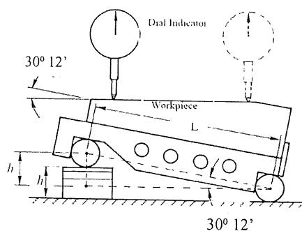
Figure 1 : Sine-bar set-up
